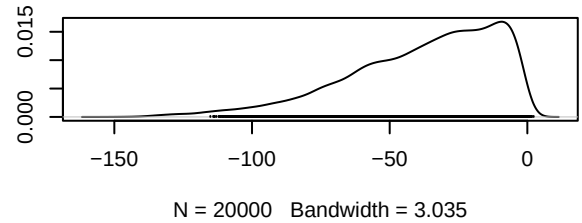
Density of d.I.I_Autophagyi
