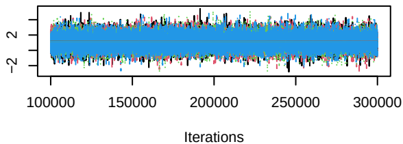
Trace of d.I.I_ERi
