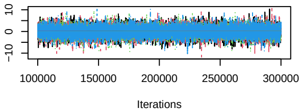
Trace of d.I.Rociletinib
