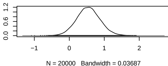
Density of d.l.chemo
