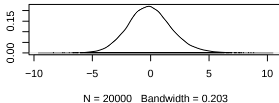
Density of d.I.I_HGFi
