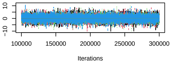
Trace of d.l.DHFRi
